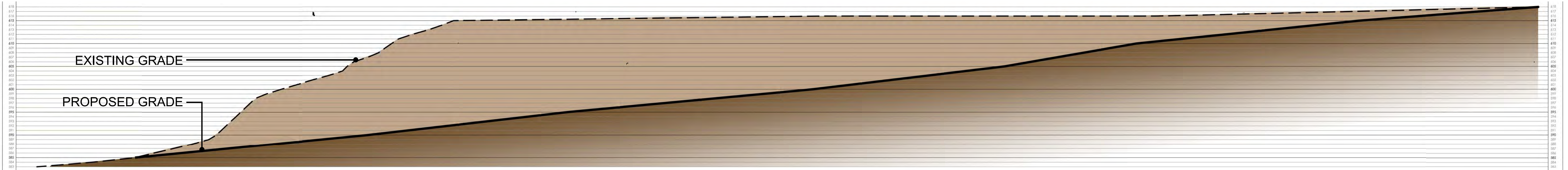
SECTION THROUGH CENTER LINE OF PROPOSED ASPHALT WALK 1" = 10'
