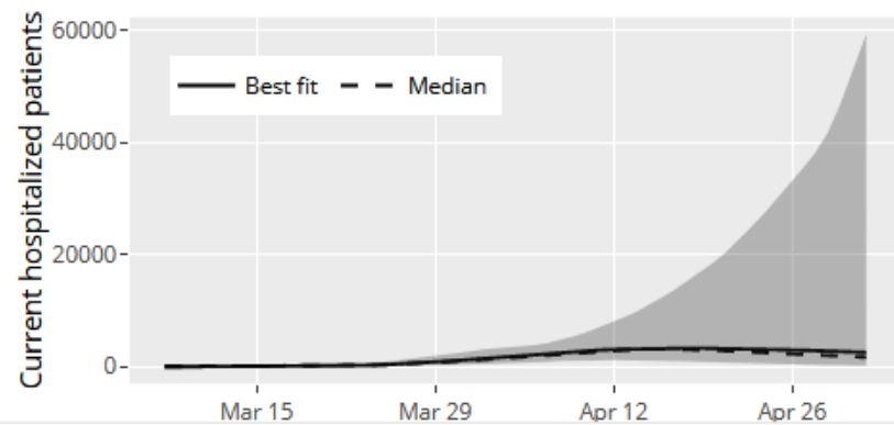
3-week forecast of COVID-19 hospitalized patients (i.e. beds needed)
