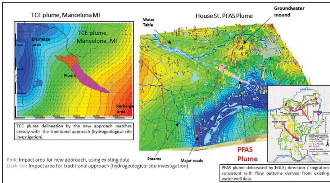
Figure 20: Examples of forward contaminant particle tracking: (left) comparison of the TCE plume in Mancelona, MI, where the red polygon is the plume delineate from traditional hydrogeological field investigation, and the pink is the envelope of simulated particle path lines; (right) House St. PFAS plume (pink polygon) and the simulated water table. Forward tracking is best used to answer: if a spill occurs, where does it go, and how long will it take?
