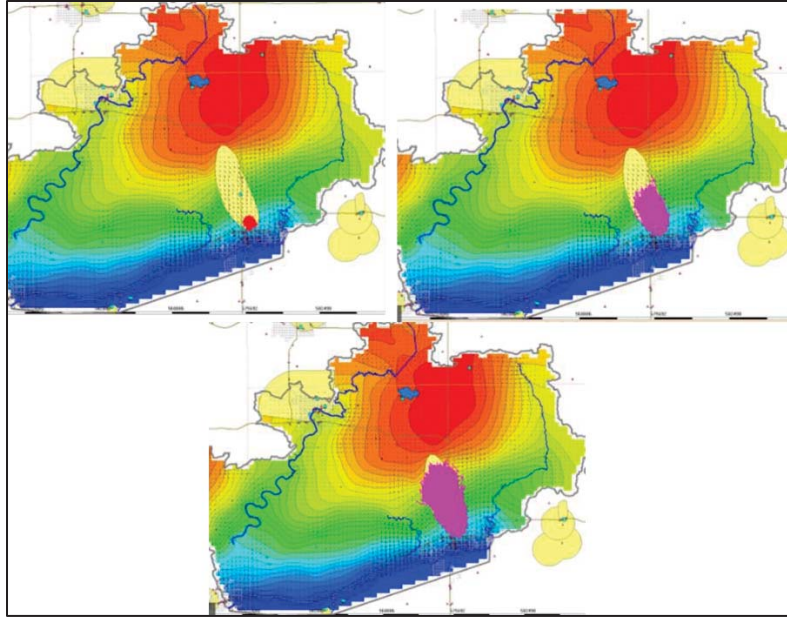
Figure 21: Example of reverse particle tracking in Kent County, MI for wellhead protection area (WHPA) delineation. The different graphics show the pathlines at different elapsed times (starting at time≈0 in the top-left). The simulated pathlines match well with the wellhead protection area delineated with traditional hydrogeological field investigations. Backward tracking is best used to determine: if a contaminant is found in a monitoring well, where does it come from (Figure 21), and how long ago was it released?
